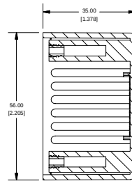
SECTION B-B SCALE 1 : 1
