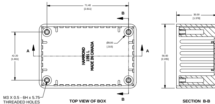
TOP VIEW OF BOX
