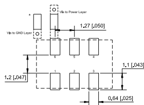
Recommended Land Pattern for LVPECL, LVDS, HCSL
