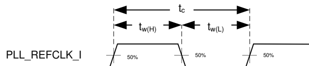
Figure 6-2. PLL Reference Clock Timing
