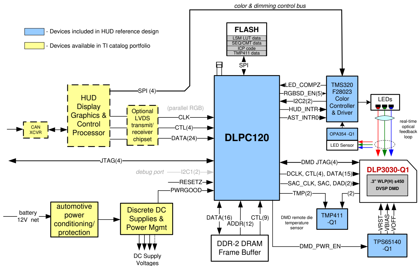
Figure 9-1. DLPC120-Q1 System Block Diagram
