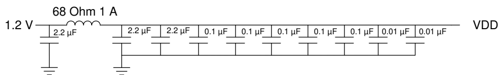
Figure 10-3. VDD Recommended Filter
