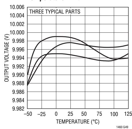
LT1460S3-10V Output Voltage Temperature Drift
