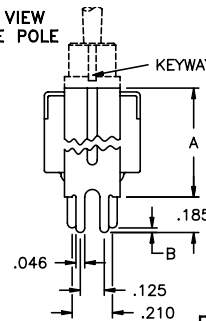
SIDE VIEW - SINGLE AND DOUBLE POLE
