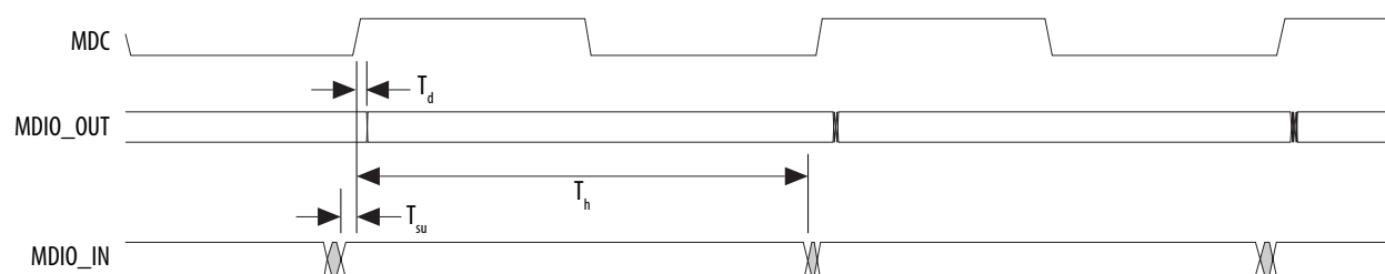
Figure 1-15: MDIO Timing Diagram
