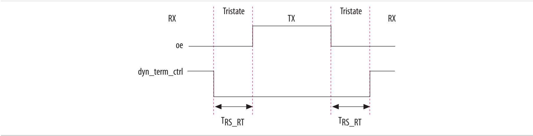
Figure 2-6: Timing Diagram for oe and dyn_term_ctrl Signals
