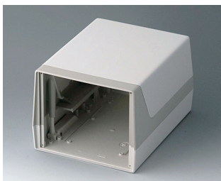
A9917837 LUX CASE 230, Vers. I ABS (UL 94 HB) off-white RAL 9002 6.81"x9.06"x5.35"
