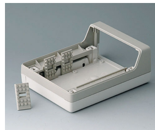
A9199000 Card guide ABS (UL 94 HB) pebble gray RAL 7032
