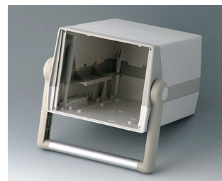
A9917857 LUX CASE 230, Vers. III ABS (UL 94 HB) off white/pebble gray RAL 9002/7032 6.81"x9.06"x5.35"
