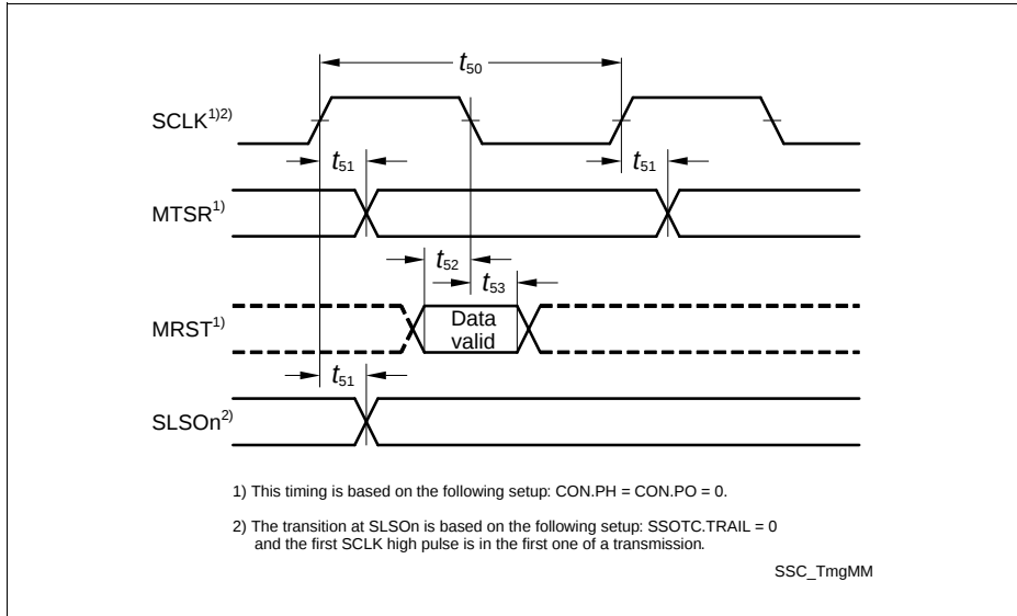
Figure 19 Master Mode Timing
