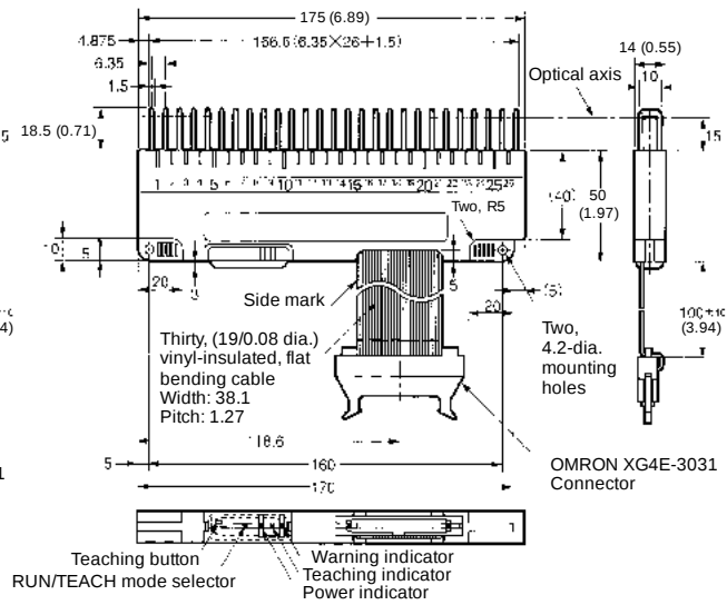
Mounting Dimensions
