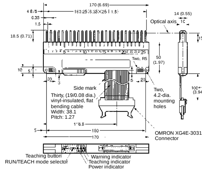
Mounting Dimensions
