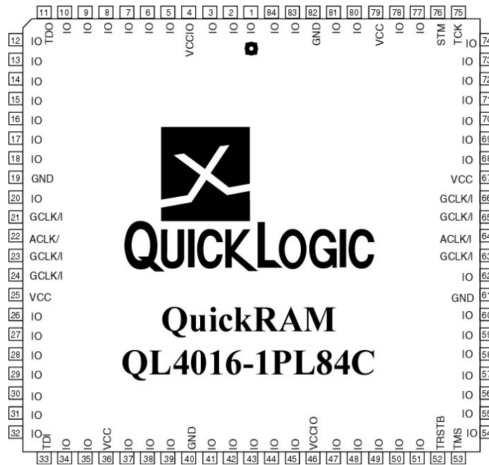
84 Pin PLCC Pinout Diagram
