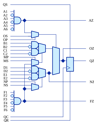
FIGURE 4. Logic Cell
