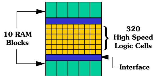
FIGURE 1. QuickRAM Block Diagram
