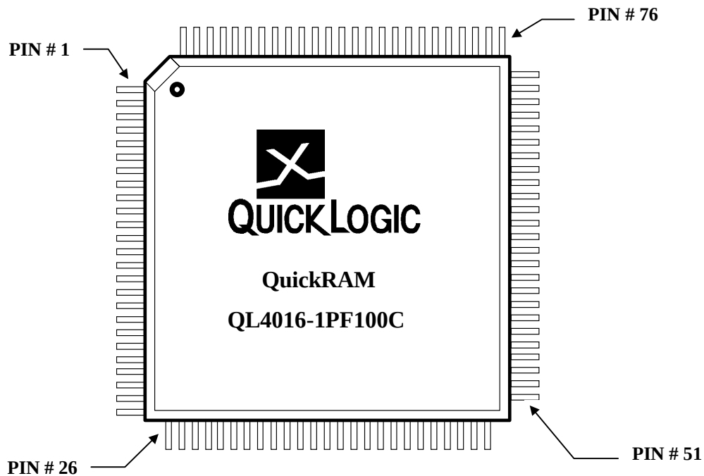
100 Pin TQFP/CQFP Pinout Diagram
