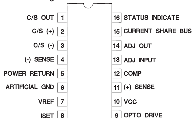
DIL-16 (Top View) J or N Package
