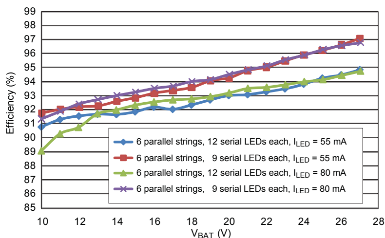
Figure 2. Efficiency versus Battery Voltage at various LED configurations, R_{FSET} = 105 \text{ k}\Omega (500 kHz), R_{ISET} = 14.3 \text{ k}\Omega (55 mA) or 10 \text{ k}\Omega (80 mA), Q1 = FQB17N08L, L1 = 10 \text{ }\mu\text{H}
