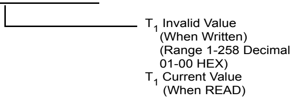
Figure 42. Counter/Timer 1 Register (F2 h : Read/Write)
