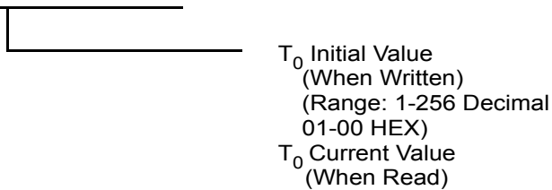
Figure 44. Counter/Timer 0 Register (F4 h : Read/Write)
