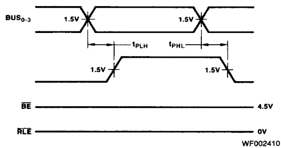
BUS TO PARITY OUTPUT
