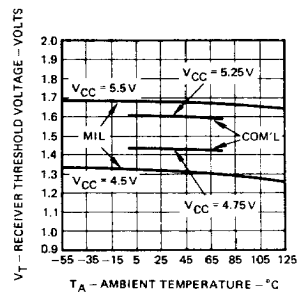
Am2908 Receiver Threshold Variation Versus Ambient Temperature
