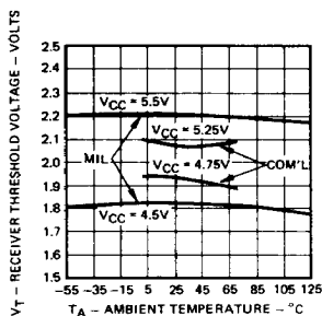
Am2907 Receiver Threshold Variation Versus Ambient Temperature
