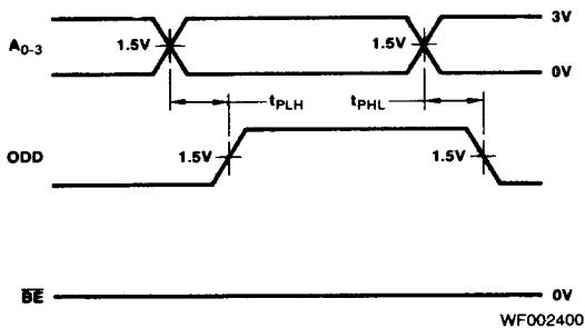
A INPUT TO PARITY OUTPUT
