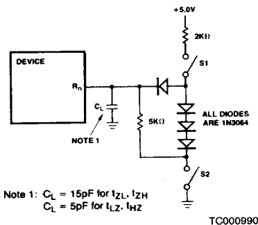
LOAD FOR RECEIVER TRI-STATE TEST
