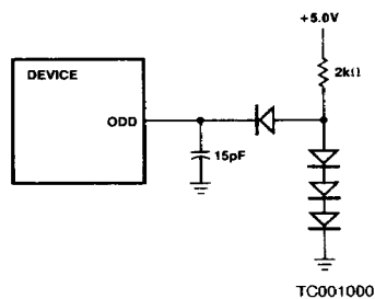
LOAD FOR PARITY OUTPUT
