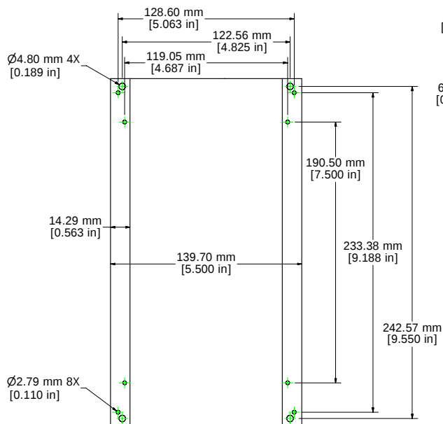
TOP PANEL - BOTTOM ENCLOSURE
