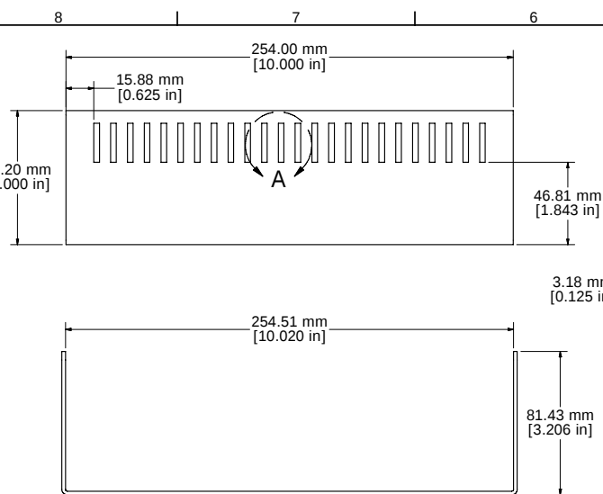
ASSEMBLY - REAR VIEW (OPEN)
