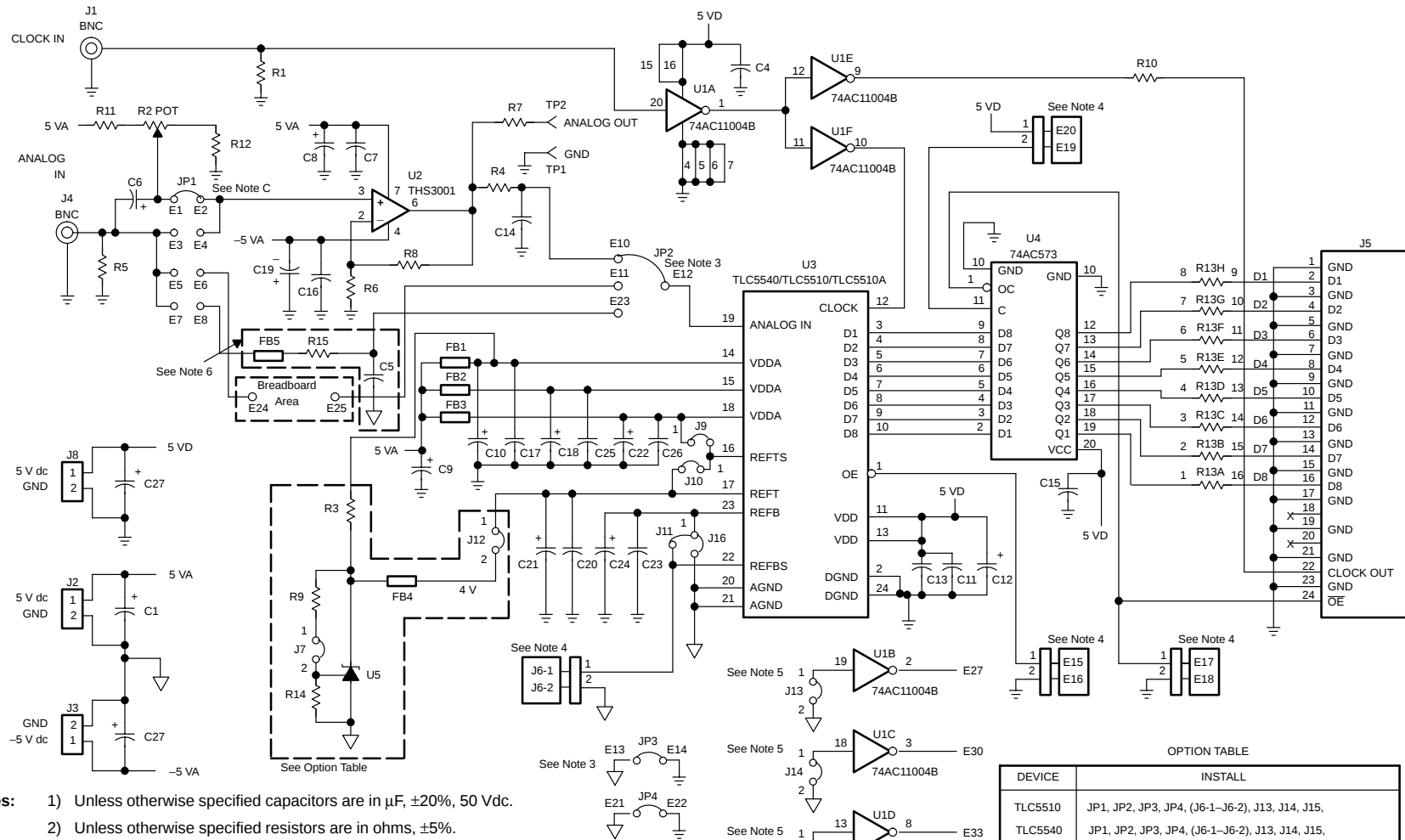
Figure 2–1. Board Schematic
