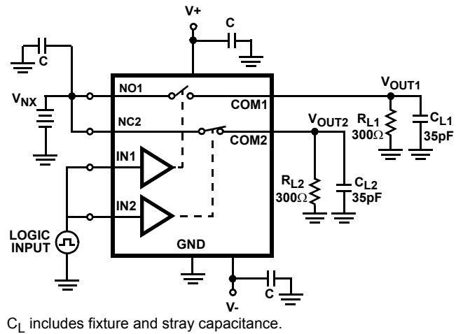
FIGURE 3B. TEST CIRCUIT
