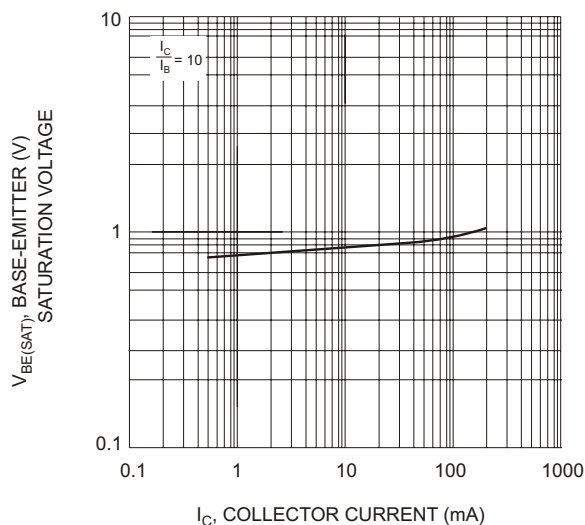
I_C , COLLECTOR CURRENT (mA) Fig. 5, Typical Base-Emitter Saturation Voltage vs. Collector Current (Transistor Element)
