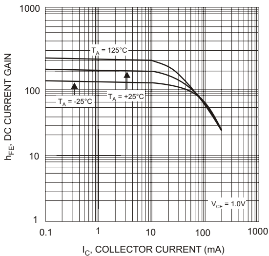
I_C , COLLECTOR CURRENT (mA) Fig. 3, Typical DC Current Gain vs Collector Current (Transistor Element)
