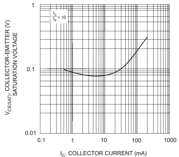
I_C , COLLECTOR CURRENT (mA) Fig. 4, Typical Collector-Emitter Saturation Voltage vs. Collector Current (Transistor Element)
