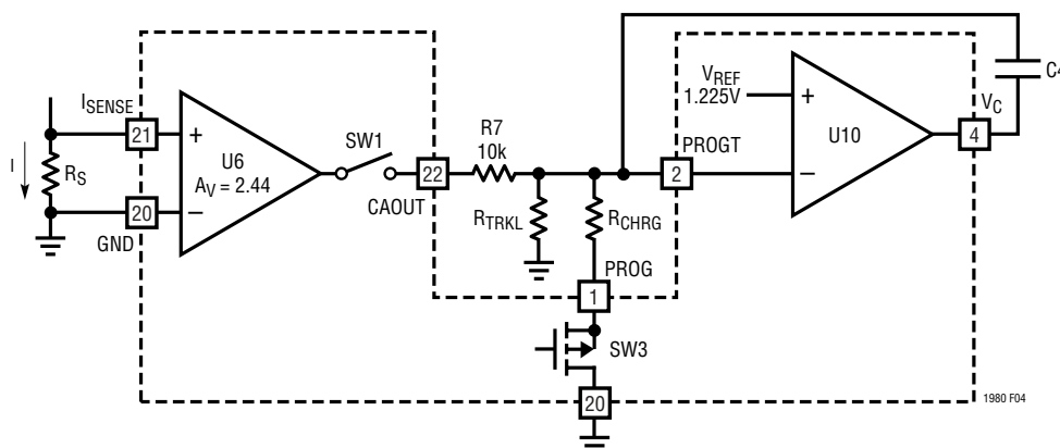
Figure 4. Battery Charger Current Control Loop
