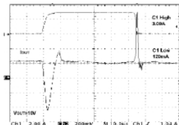
Figure 23: Load Transient
