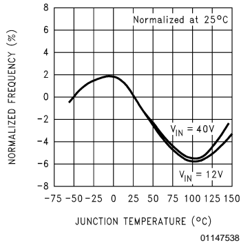
Oscillator Frequency
