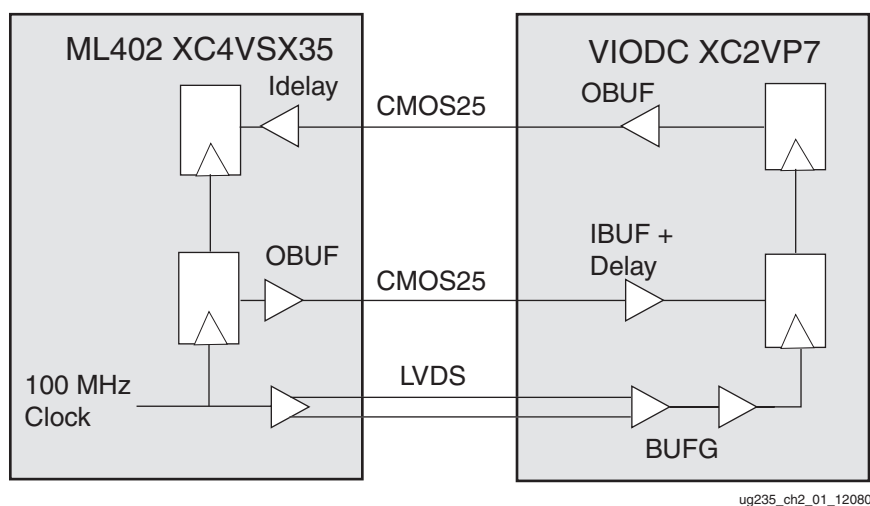
Figure 2-1: VIOBUS Clocking
