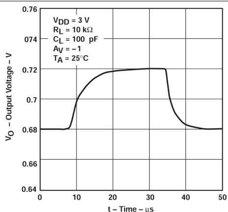
Figure 5-25. Inverting Small-Signal Pulse Response
