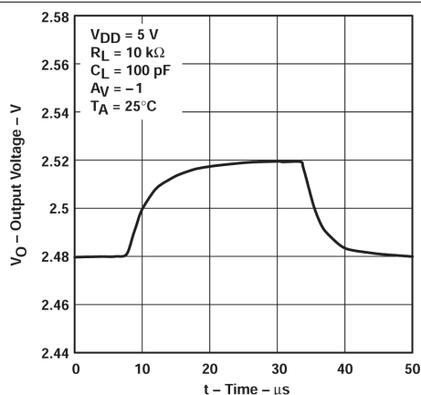
Figure 5-26. Inverting Small-Signal Pulse Response
