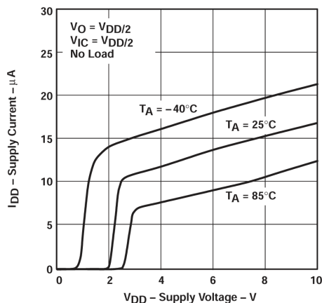
Figure 5-19. Supply Current vs Supply Voltage
