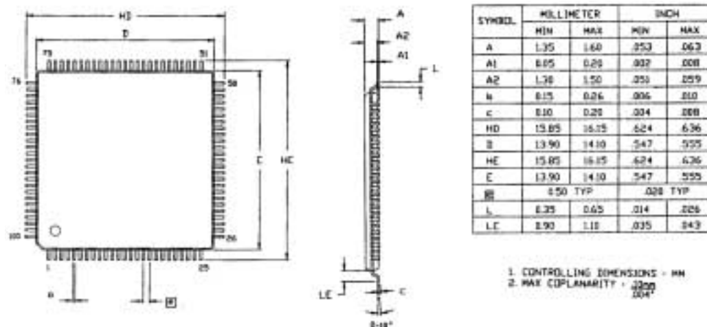
Figure 18. 100-Lead Plastic Very Small Quad Flatpack (VQFP)
