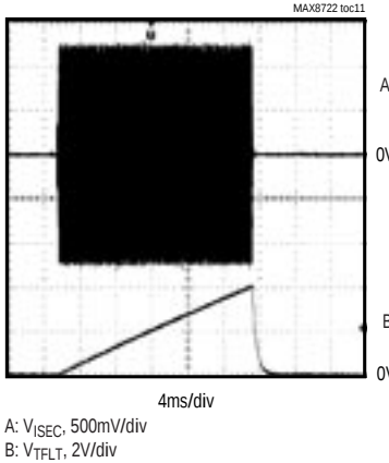
SECONDARY OVERCURRENT PROTECTION AND TIMEOUT
