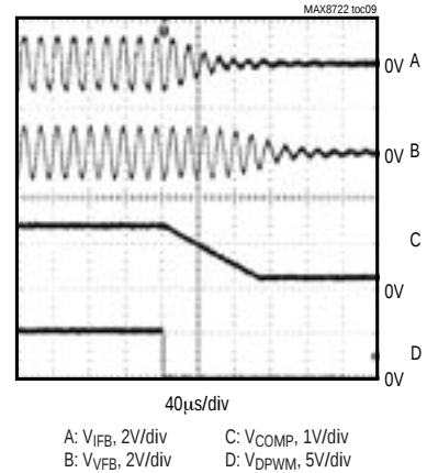
DIGITAL PWM SOFT-STOP
