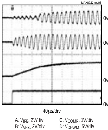
DIGITAL PWM SOFT-START
