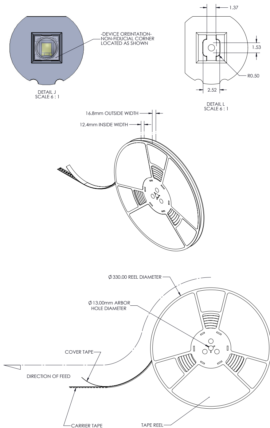
Figure 11: Reel dimensions for LUXEON T.
