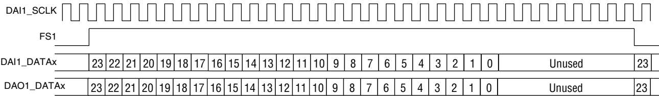
Figure 12. Audio Data Timing Detail - Standard Mode, 64FS - CS18100x/CS49610x, CS18101x/CS49611x
