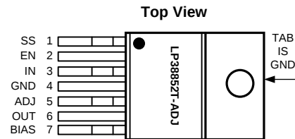
Figure 2. TO-220-7 Package See Package Number NDZ0007B
