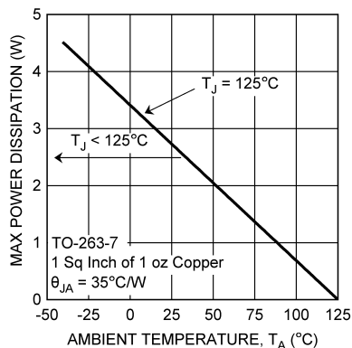
Figure 34. Maximum Power Dissipation vs Ambient Temperature for the DPAK Package
