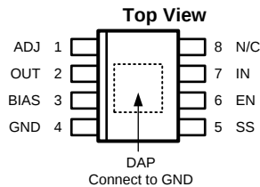
Figure 3. SO PowerPAD-8 Package See Package Number DDA0008A
