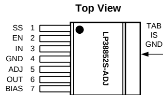
Figure 1. DDPAK-7 Package See Package Number KTW0007B
