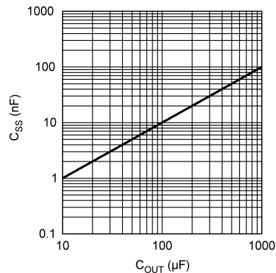
Figure 32. Typical C SS vs C OUT Values
