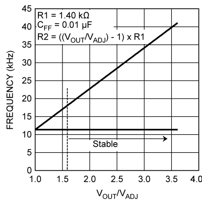
Figure 31. F_{ZERO} and F_{POLE} vs Gain
