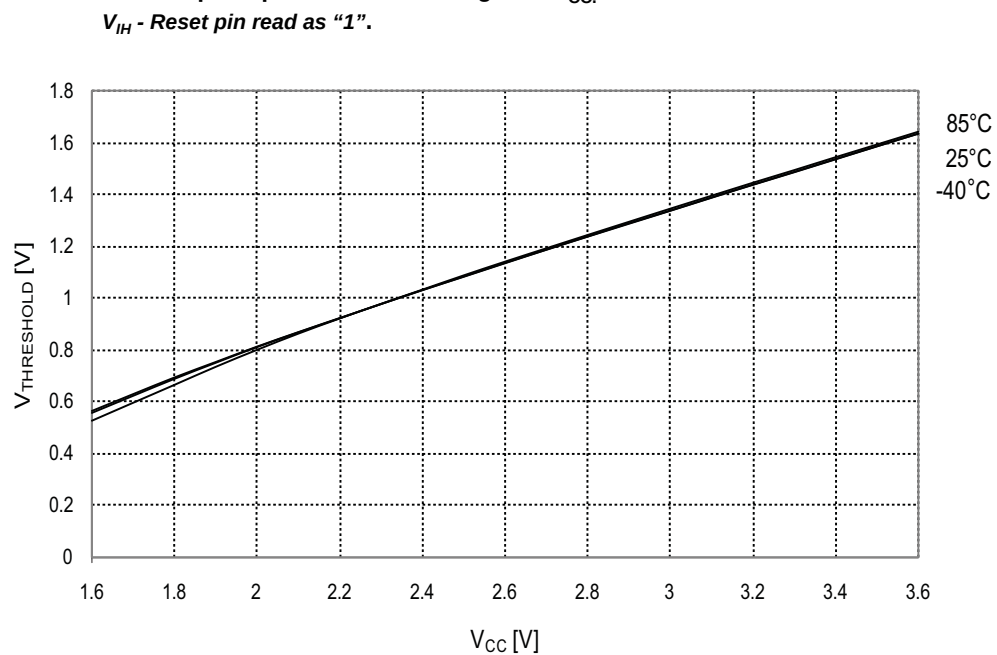
Figure 34-188. Reset pin input threshold voltage vs. V_{CC} .
