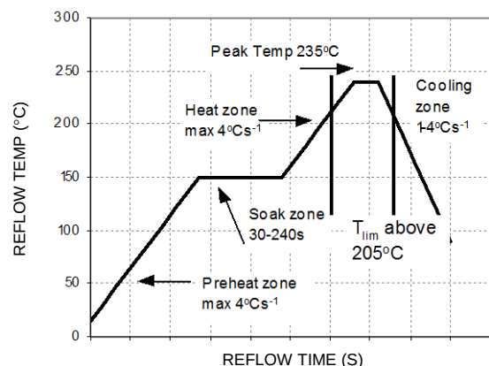
Figure 72. Recommended Reflow Profile
