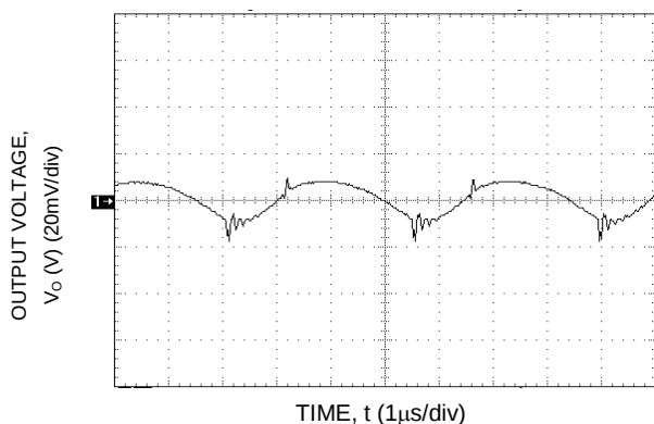
Figure 44. Typical Output Ripple and Noise.
