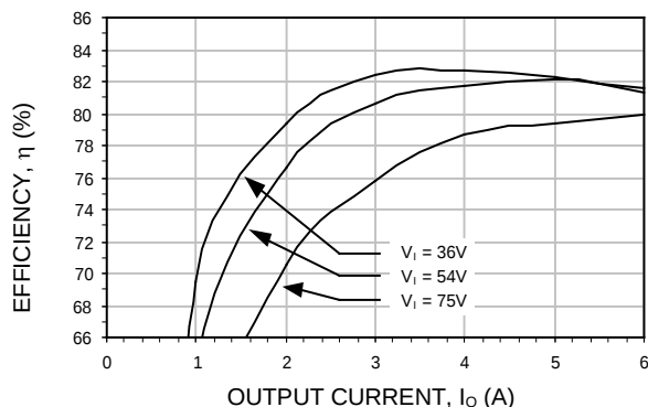
Figure 25. Converter Efficiency versus Output Current
