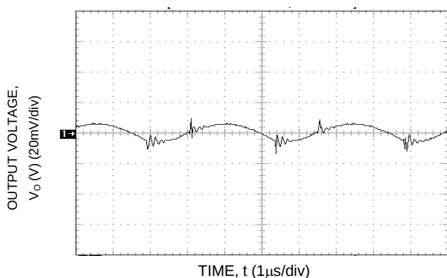
Figure 32. Typical Output Ripple and Noise.
