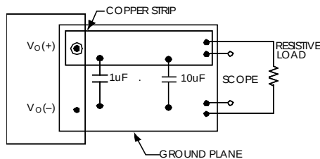
Figure 61. Input Reflected Ripple Current Test Setup.
