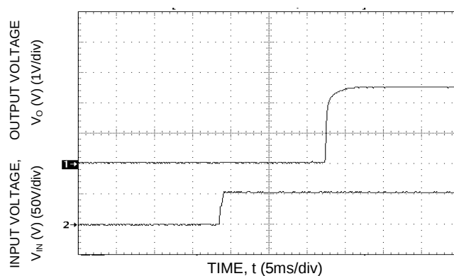
Figure 17. Typical Start-Up with application of V_{in} .
