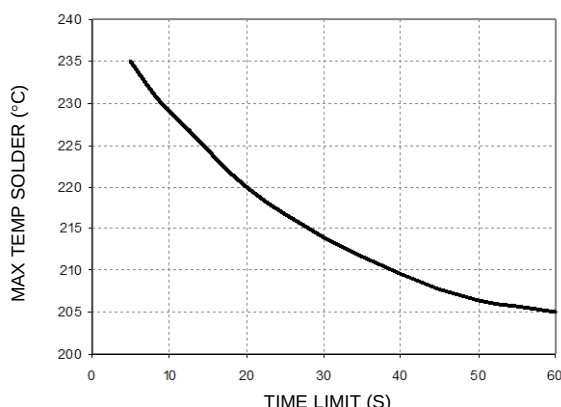
Figure 73. Time Limit Curve Above 205°C Reflow .
