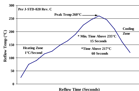
Figure 74. Recommended linear reflow profile using Sn/Ag/Cu solder.
