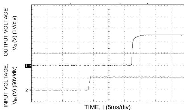
Figure 17. Typical Start-Up with application of V_{in} .
