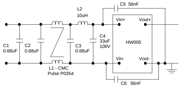
Figure 67. Suggested Configuration for EN55022 Class B.
