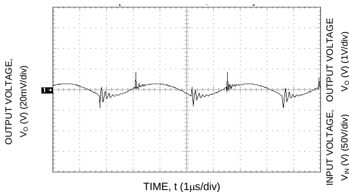
Figure 8. Typical Output Ripple and Noise.
