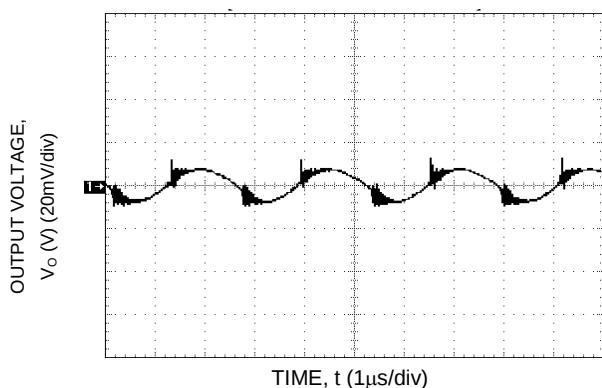
Figure 50. Typical Output Ripple and Noise.
