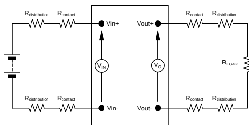
Figure 62. Output Ripple and Noise Test Setup.
