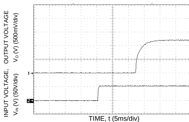
Figure 41. Typical Start-Up with application of Vin.
