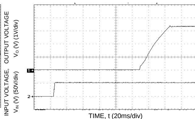
Figure 11. Typical Start-Up with application of V_{in} .
