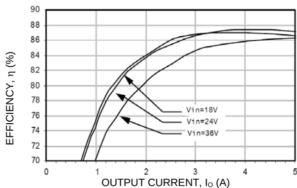
Figure 55. Converter Efficiency versus Output Current.
