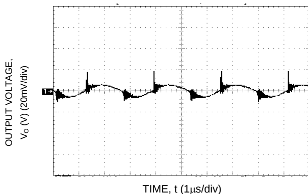
Figure 56. Typical Output Ripple and Noise.
