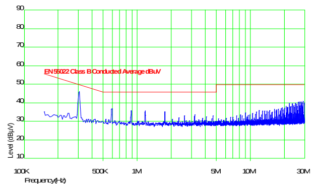
Figure 68. EMC signature using above filter, HW005A0F.
