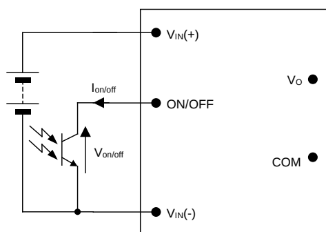
Figure 64. Remote On/Off Implementation.
