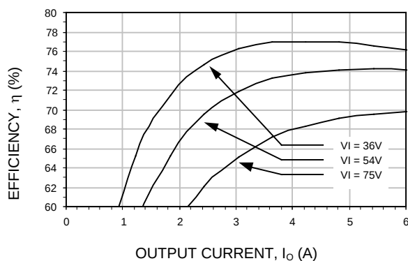
Figure 43. Converter Efficiency versus Output Current.
