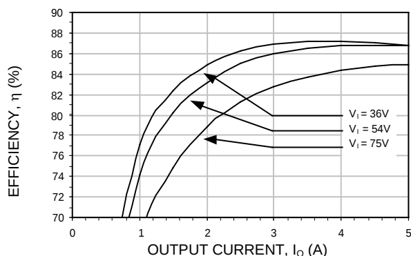
Figure 7. Converter Efficiency versus Output Current
