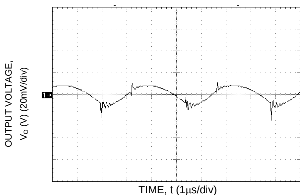
Figure 38. Typical Output Ripple and Noise.
