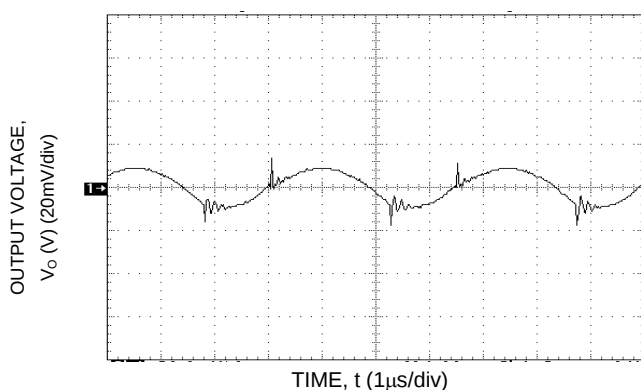
Figure 14. Typical Output Ripple and Noise.
