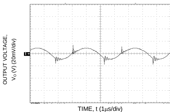
Figure 14. Typical Output Ripple and Noise.
