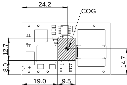
Figure 70. Pick and Place Location.
