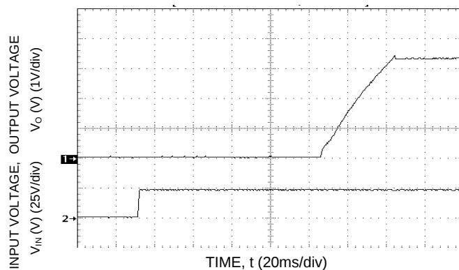
Figure 59. Typical Start-Up with application of V_{in} .
