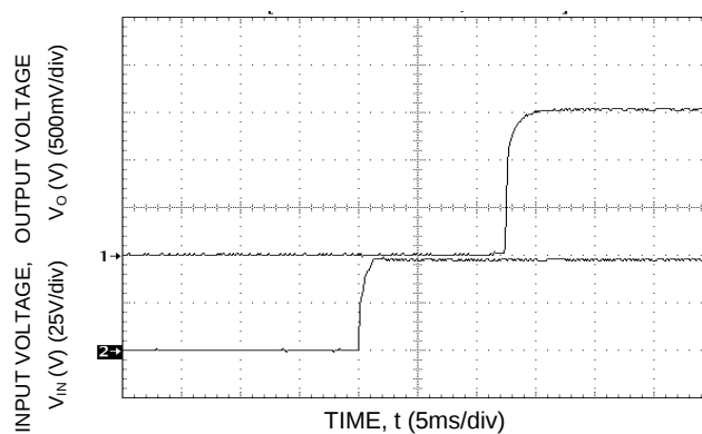
Figure 35. Typical Start-Up with application of Vin.
