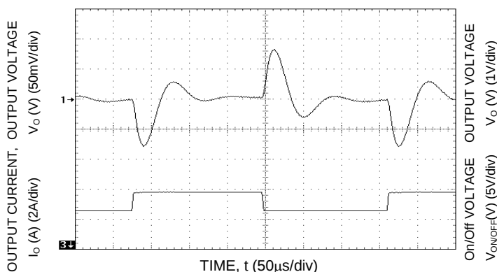
Figure 9. Transient Response to Dynamic Load Change from 50% to 75% to 50% of full load.
