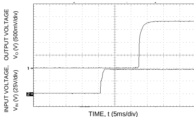
Figure 29. Typical Start-Up with application of V_{in} .
