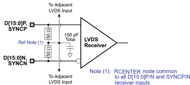
Figure 26. D[15:0]P/N and SYNC/N LVDS Input Configuration
