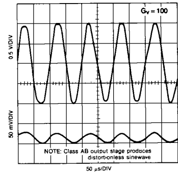
Figure 2. Wave Response
