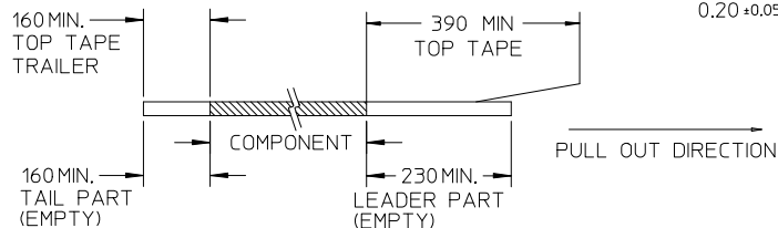
DETAIL 1
