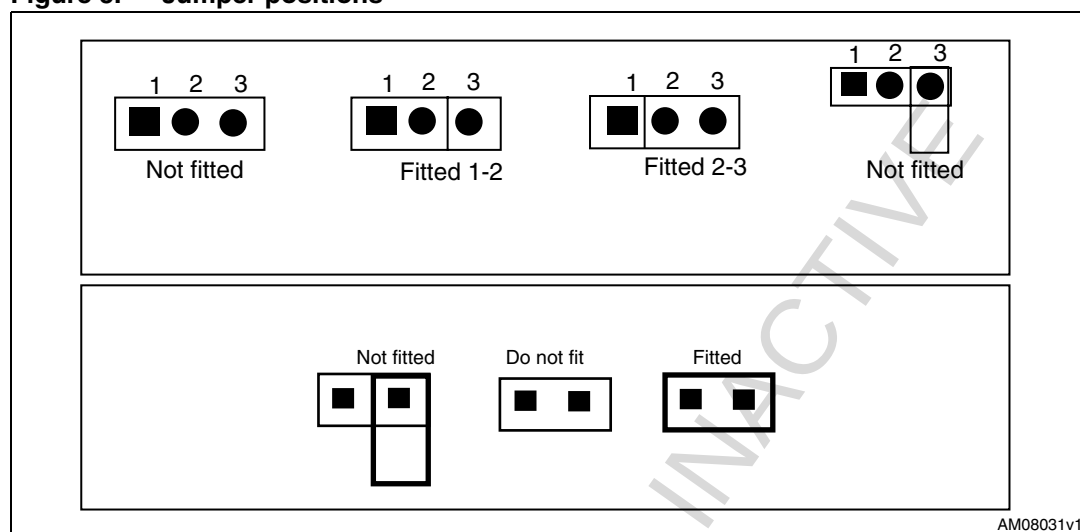
Figure 5. Jumper positions
