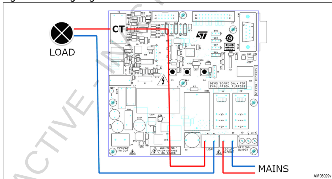
Figure 3. Wiring diagram
