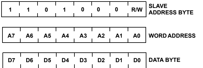
FIGURE 13. SLAVE ADDRESS, WORD ADDRESS, AND DATA BYTES
