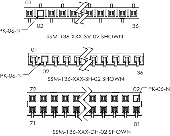
FIG 7 POLARIZATION (DIFFERENT AS SHOWN, OTHERWISE SAME AS FIG 1)
