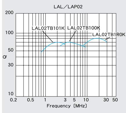
Q-周波数特性例 Q-Characteristics(Measured by HP4342A)
