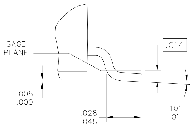
DETAIL "D"
