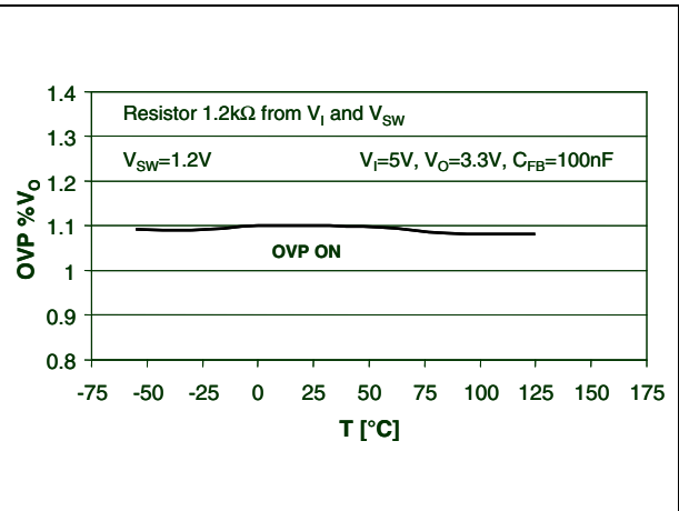
Figure 16. Over voltage protection vs. temperature
