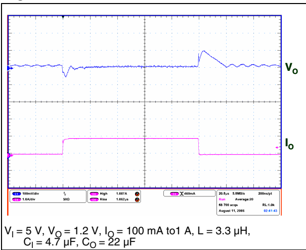
Figure 19. Load transient
