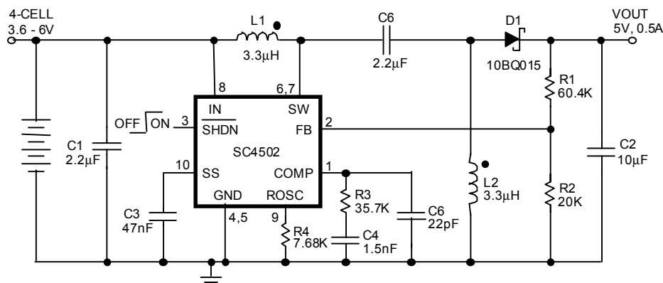
Figure 11(a). 1.5 MHz All Ceramic Capacitor 4-Cell to 5V SEPIC Converter.
