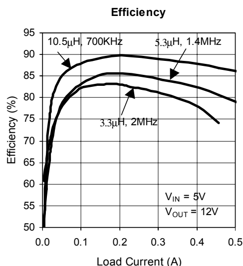
Figure 1(b). Efficiencies of 5V to 12V Boost Converters at 700KHz, 1.4MHz and 2MHz.
