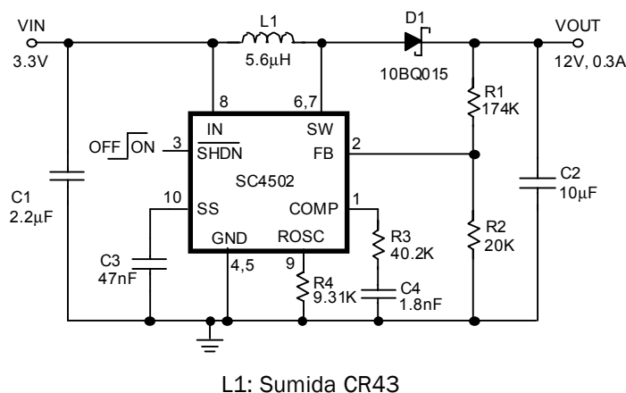
Figure 9(a). 1.35 MHz All Ceramic Capacitor 3.3V to 12V Boost Converter.
