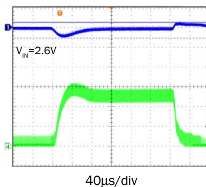
Figure 10(c). Load Transient Response of the Circuit in Figure 10(a). I_{LOAD} is switched between 90mA and 0.5A at 1A/μs.
