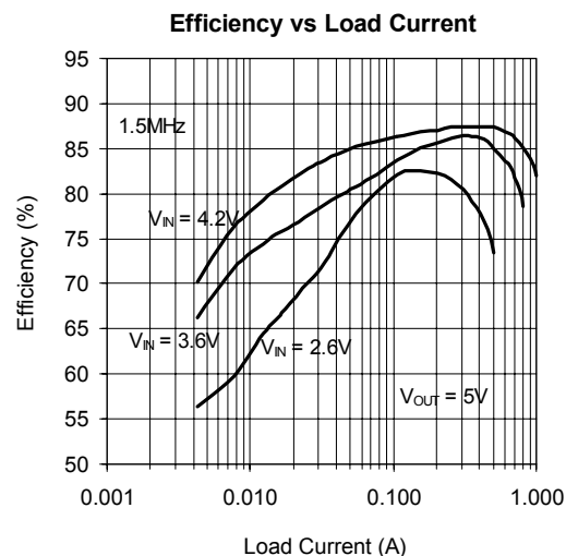
Figure 10(b). Efficiency of the Single Li-ion Cell to 5V Boost Converter in Figure 10(a).
