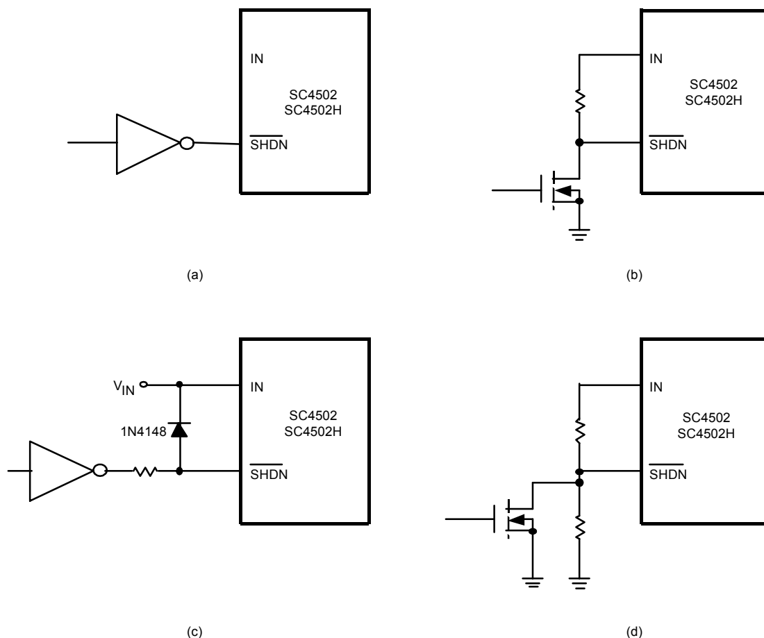
Figure 5. Methods of Driving the Shutdown Pin
