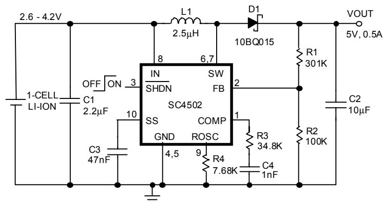
Figure 10(a). 1.5 MHz All Ceramic Capacitor Single Li-ion Cell to 5V Boost Converter.
