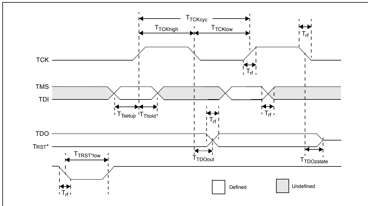
FIGURE 26-14: EJTAG TIMING CHARACTERISTICS
