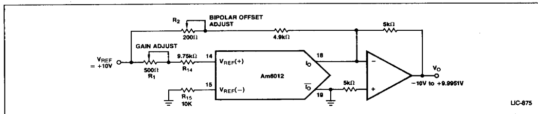
Figure 14. \pm 10\text{V} Full-Scale Bipolar DAC
