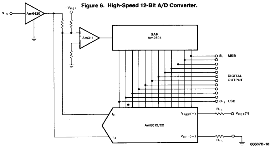
Figure 6. High-Speed 12-Bit A/D Converter.
