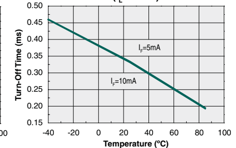
Typical Turn-Off Time vs. Temperature ( I_L=60\text{mA} )
