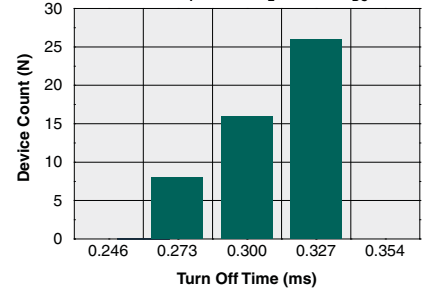
Typical Turn-Off Time (N=50, I_F=5\text{mA} , I_L=100\text{mA}_{DC} )
