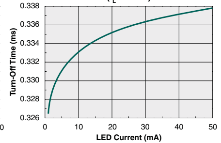
Typical Turn-Off Time vs. LED Forward Current ( I_L=60\text{mA} )
