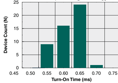
Typical Turn-On Time (N=50, I_F=5\text{mA} , I_L=100\text{mA}_{DC} )
