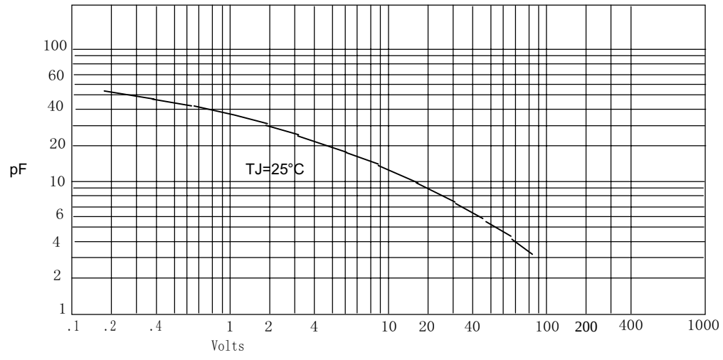
Figure 4 Junction Capacitance
