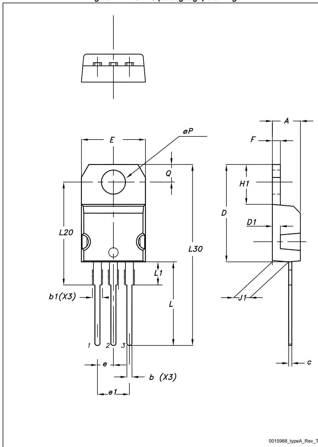
Figure 21. TO-220 (dual gauge) drawing
