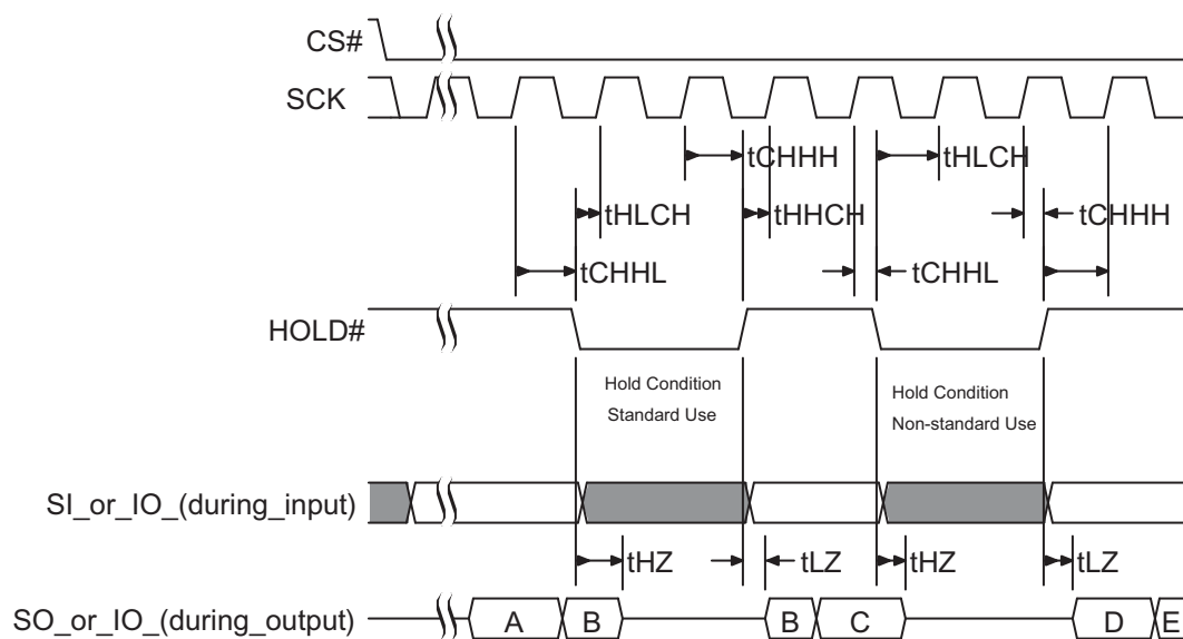
Figure 34. Hold Timing
