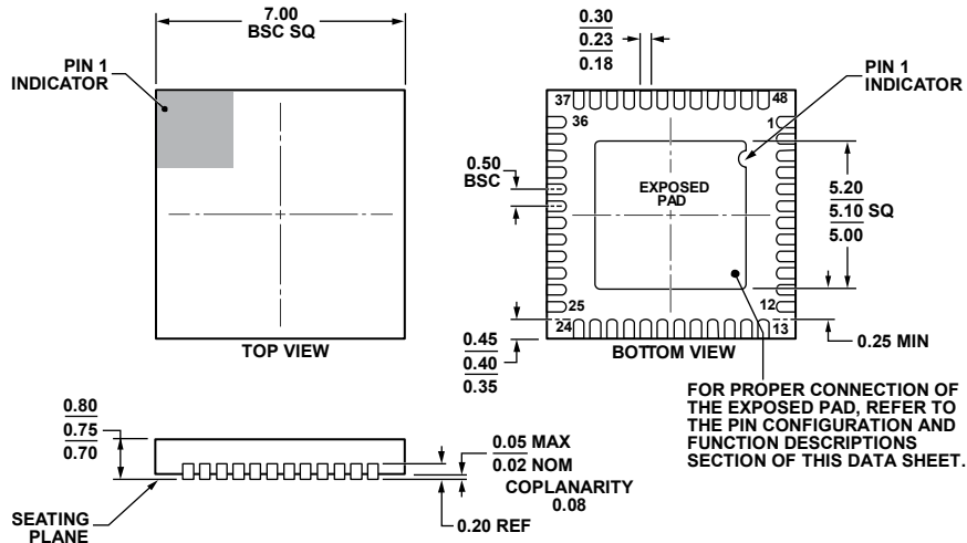
Figure 19. 48-Lead Lead Frame Chip Scale Package [LFCSP_WQ] 7 mm × 7 mm Body, Very Very Thin Quad (CP-48-4) Dimensions shown in millimeters
