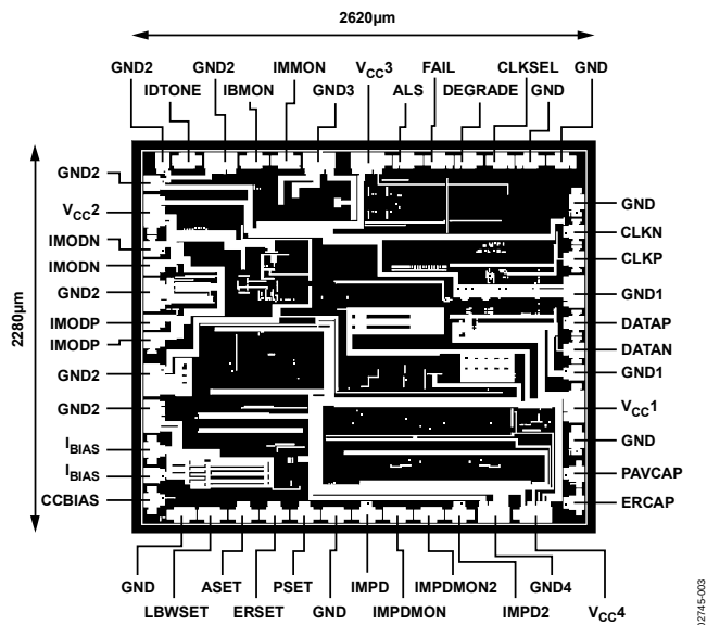
Figure 5. Metallization Photograph
