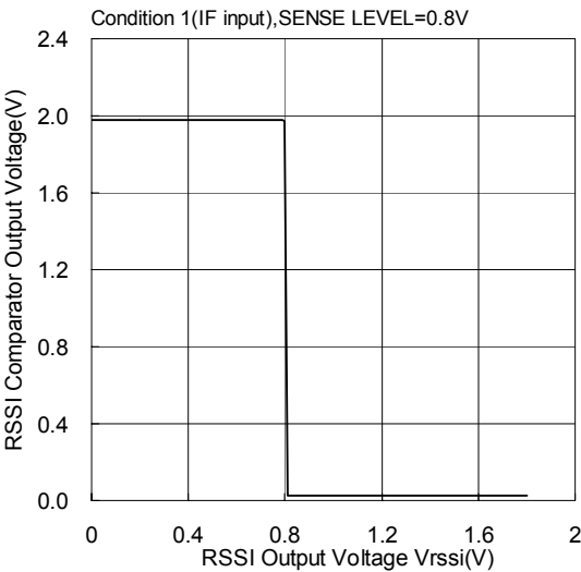
Carrier Sense Characteristics
