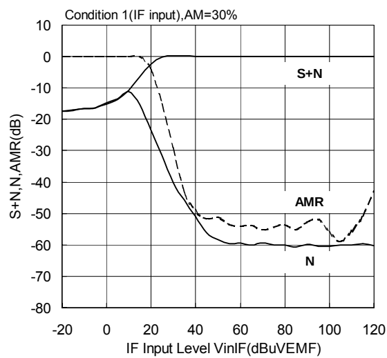
S+N,N,AMR versus IF Input
