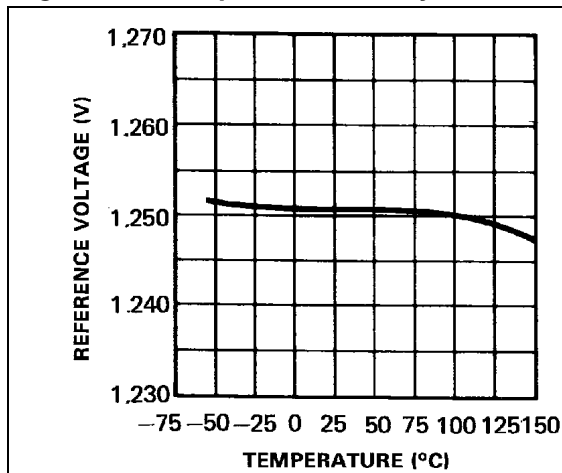
Figure 7. Temperature stability
