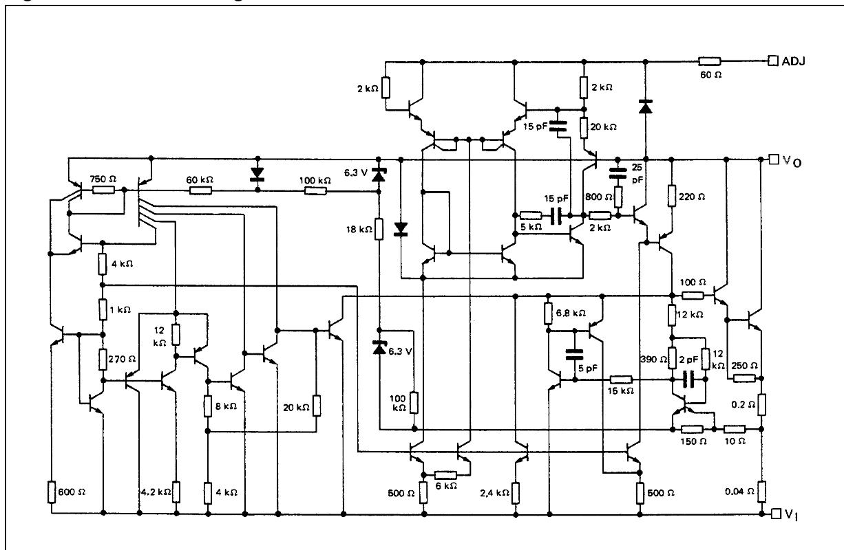
Figure 1. Schematic diagram
