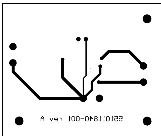
Figure 38. Bottom Layer
