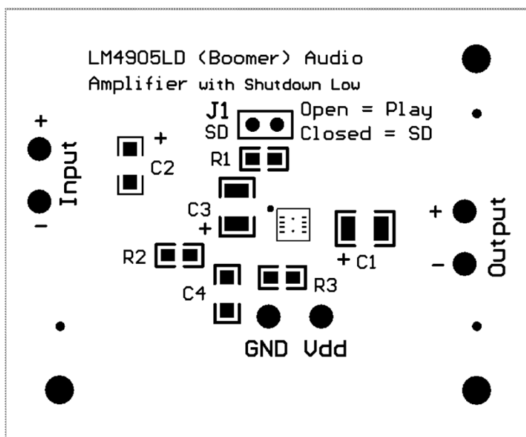
Figure 36. Silk Screen
